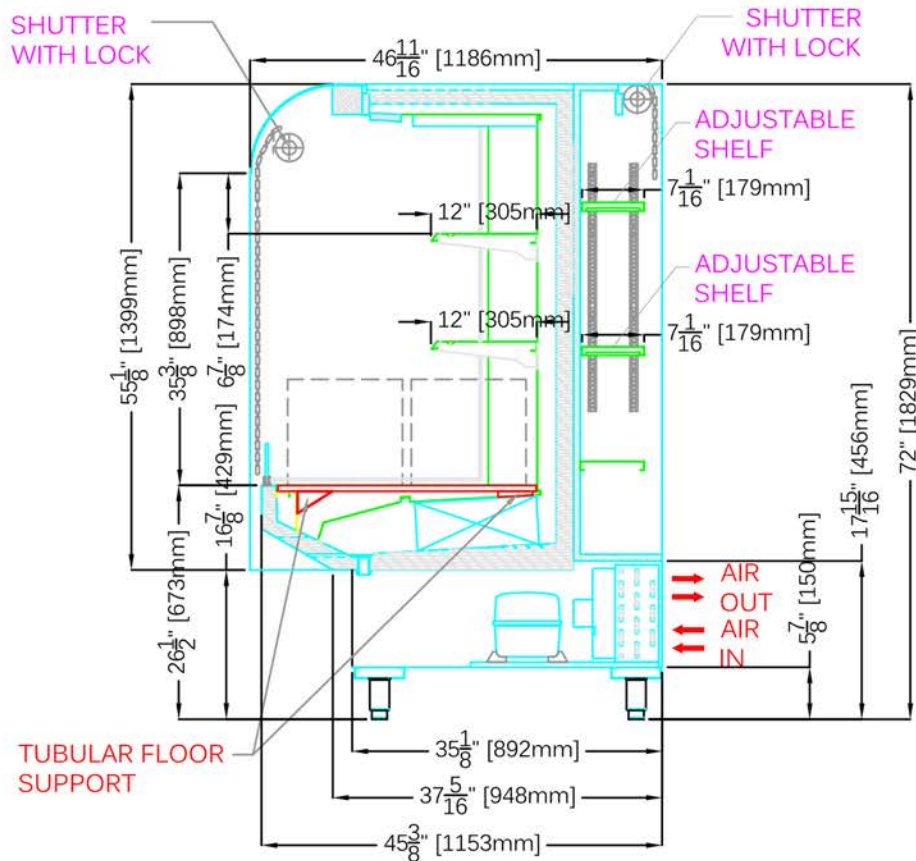
SECTION VIEW
