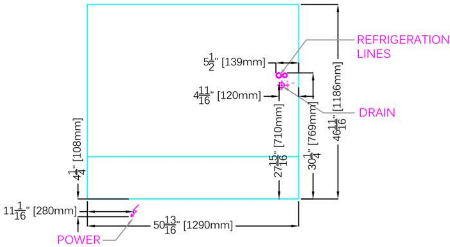
PLAN VIEW (OPERATOR SIDE)
