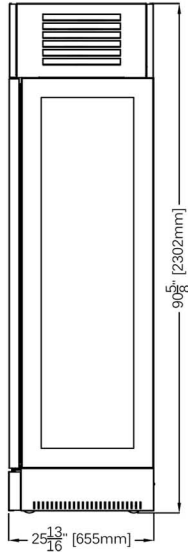
RIGHT SIDE
