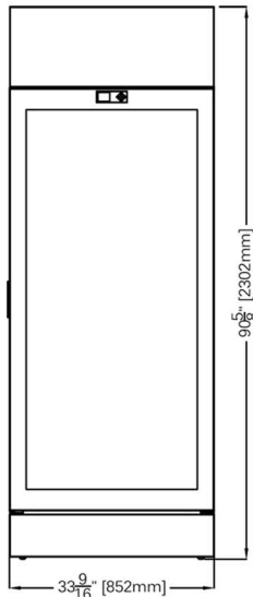
FRONT VIEW
