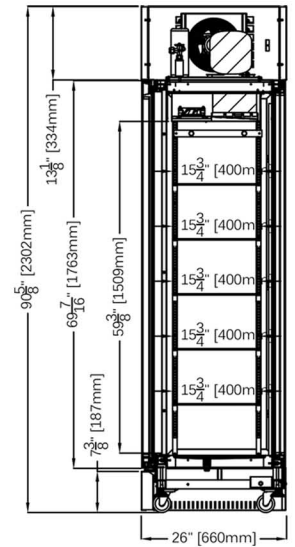
SECTION VIEW
