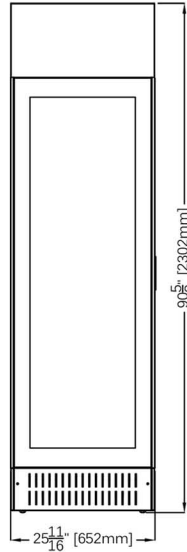
BACK VIEW
