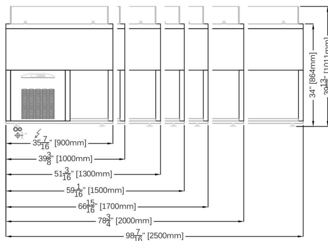
REAR ELEVATIONS (OPERATOR SIDE)
