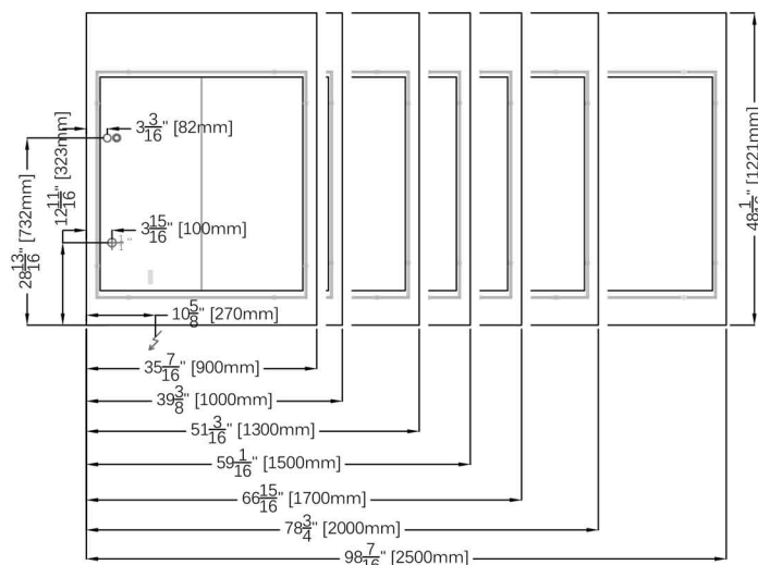
PLAN VIEWS (CUSTOMER SIDE)
