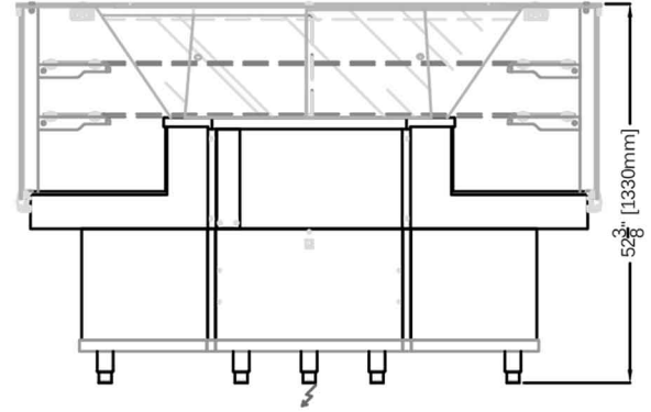
REAR ELEVATION (OPERATOR SIDE) A90 CURVE FOOTPRINT
