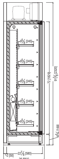
OPTIONAL: TOP MOUNTED CONDENSING UNIT
