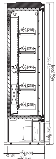
OPTIONAL: SLIDING DOORS ONLY IN SOLID SIDES AND 2100, 2800 MODELS
