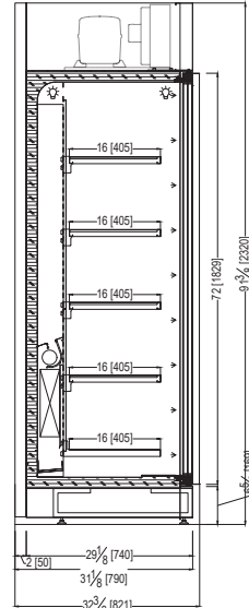
OPTIONAL: TOP MOUNTED CONDENSING UNIT
