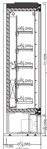
OPTIONAL: SLIDING DOORS ONLY IN SOLID SIDES AND 2100, 2800 MODELS
